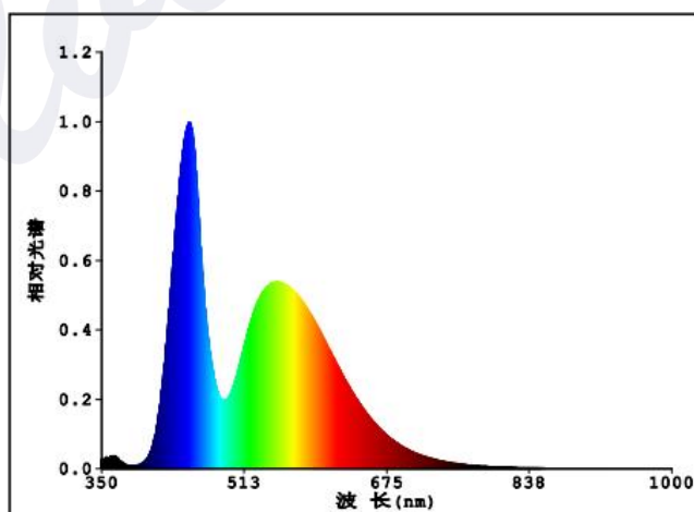
Spectral wavelength
