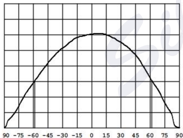
Luminous angle
